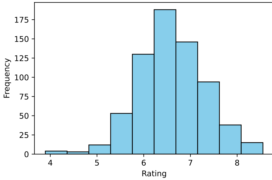
Figure 1: Rating Histogram for Genre
